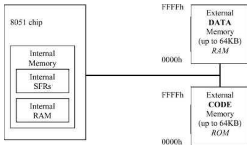
Figure 1.7: Memory representation of 8051 Microcontroller.
