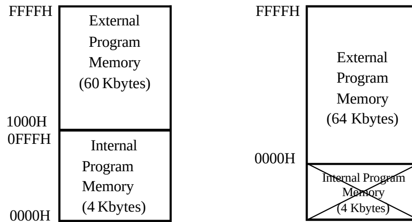
Figure . ROM Memory representation of 8051.
